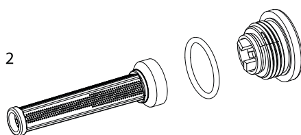
Pilot Filter Screen Assembly
