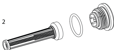
Pilot Filter Screen Assembly
